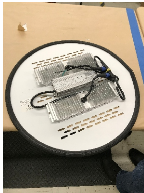
Fig 6. Install rubber gasket on retrofit fixture. Ribbed side to be on inside.
